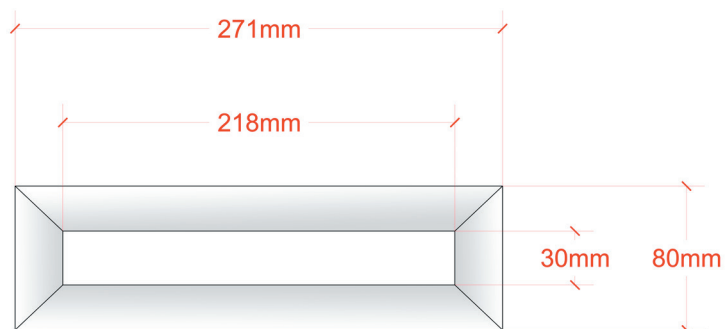
Figure 1.3 (Vent Size)
