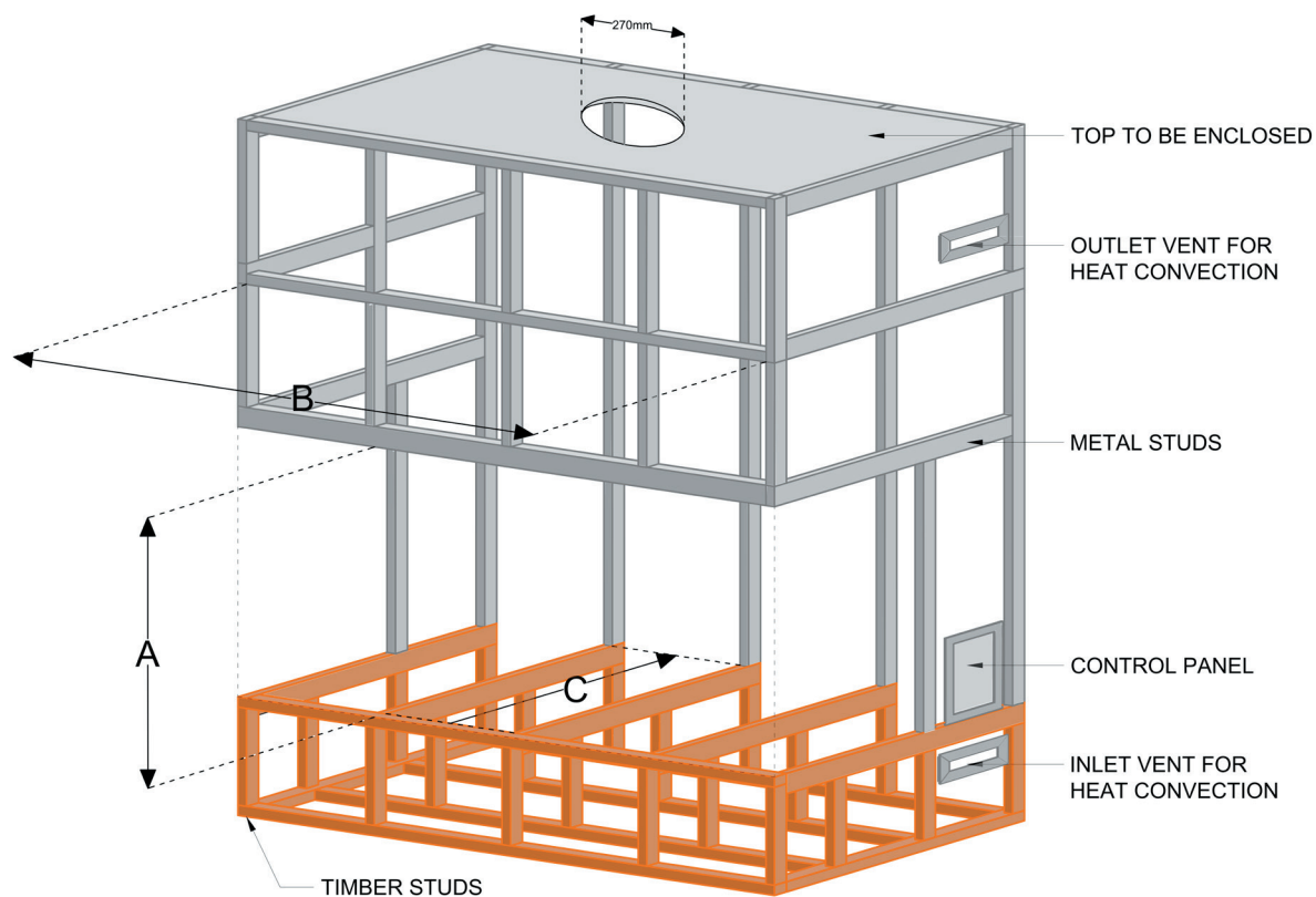
Figure 1.9 (Metal framing)
