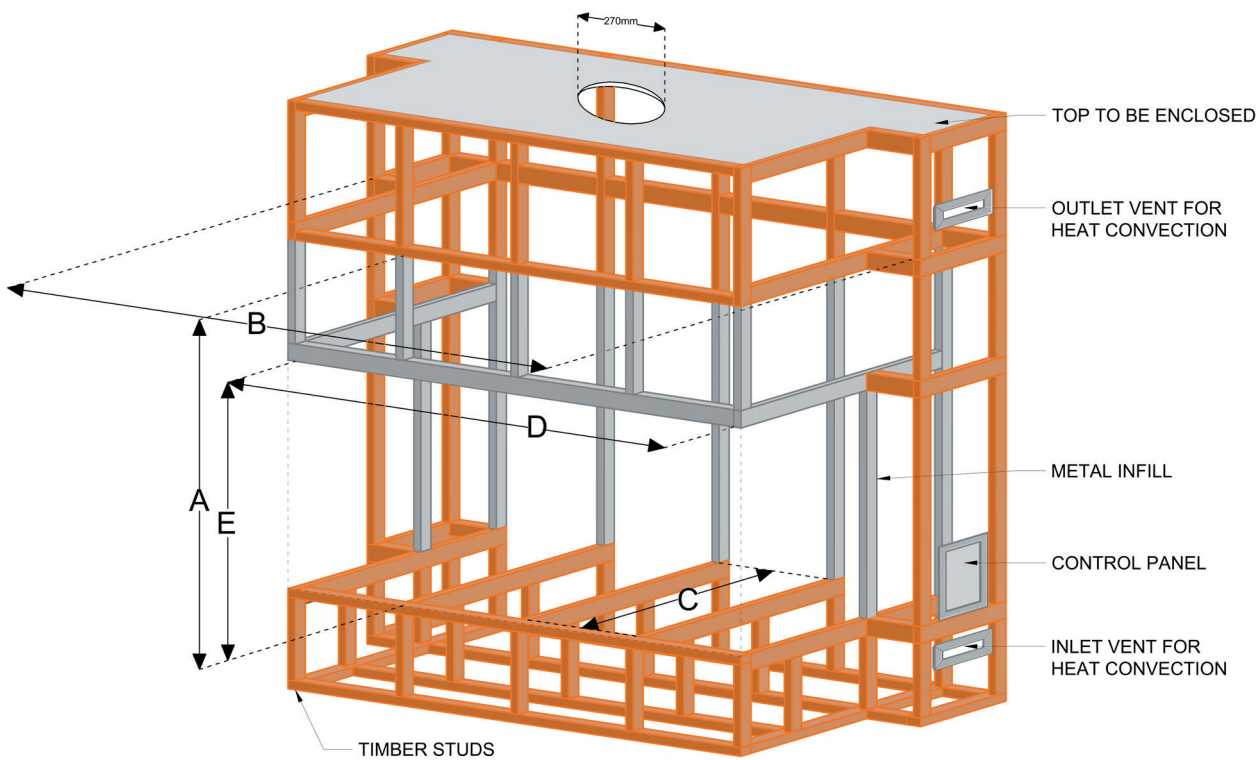
Figure 1.8 (Timber framing)
